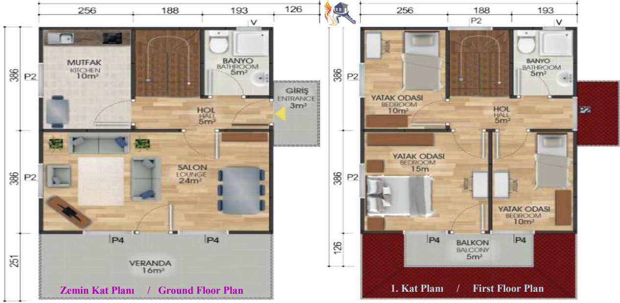
Zemin Kat Planı / Ground Floor Plan
