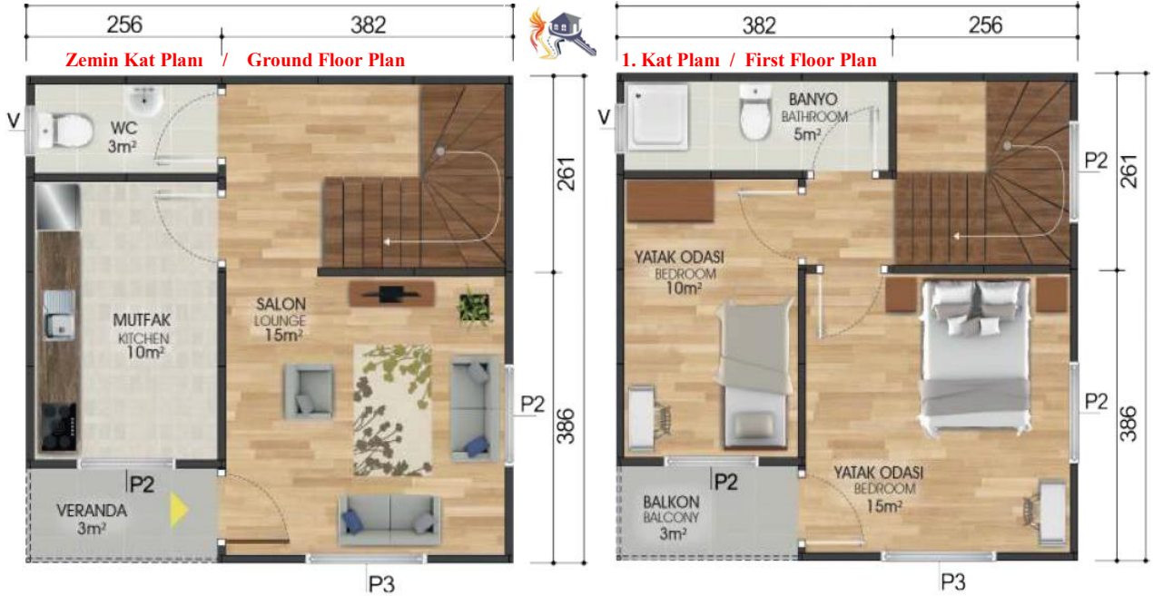
Zemin Kat Planı / Ground Floor Plan
